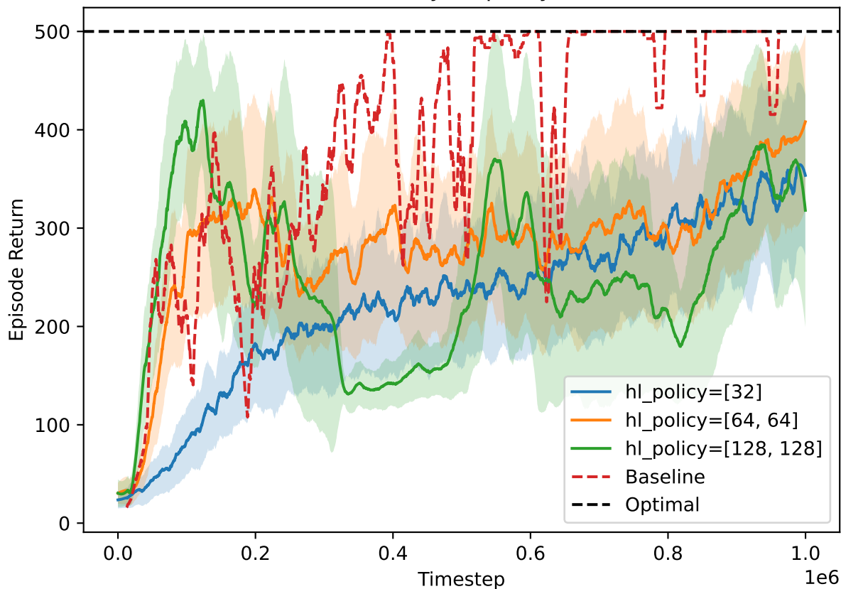
A2C hidden layers policy network
